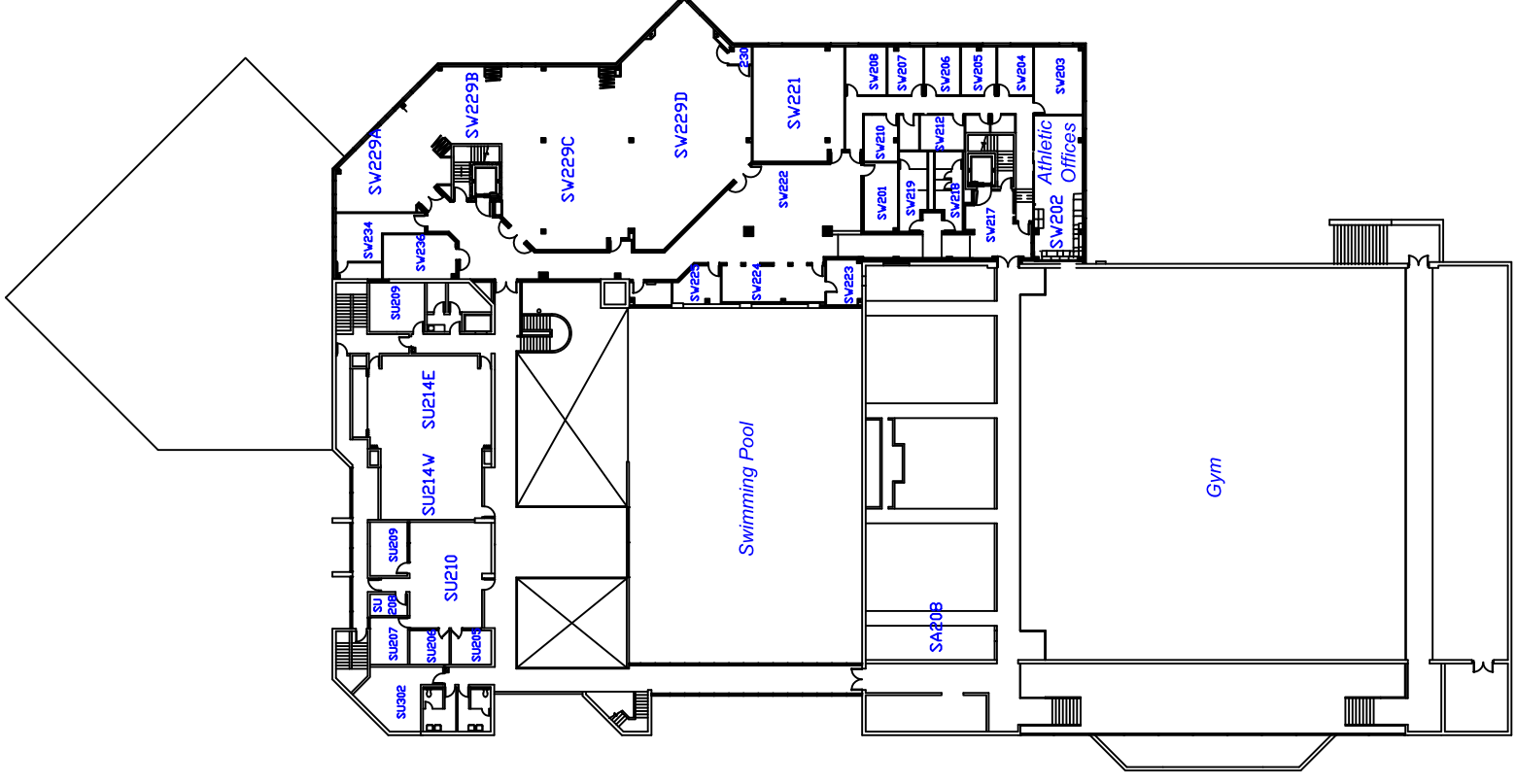
SECOND FLOOR
